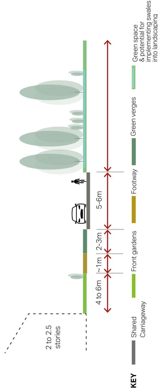
Figure 113: Illustrative section of an edge lane typology, with guide dimensions.
