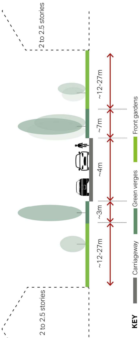
Figure 110: Illustrative section of a residential street typology, with guide dimensions, for Durfold Wood.
