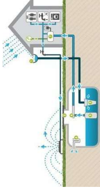
Figure 164: Diagram illustrating rainwater harvesting systems that could be integrated into open space and residential developments.
