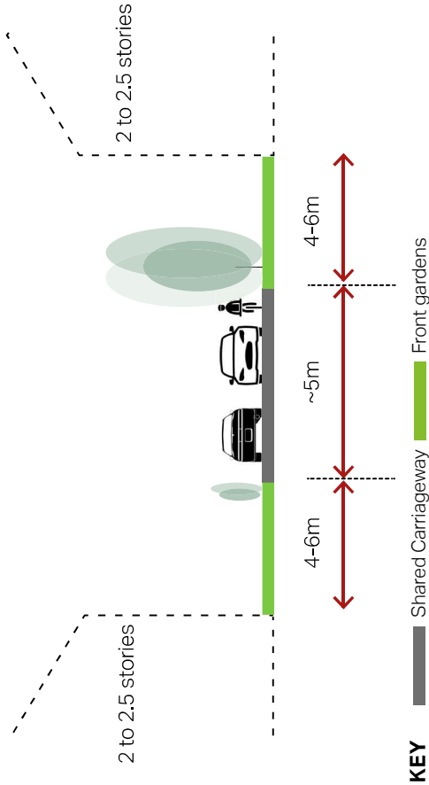
Figure 115: Illustrative section of a private lane typology, with guide dimensions.
