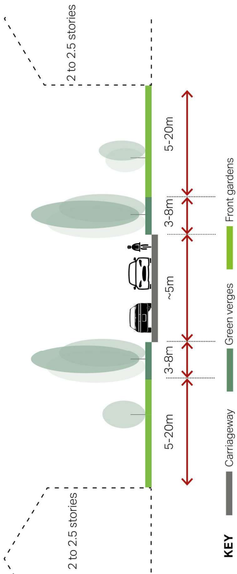
Figure 112: Illustrative section of a residential street typology, with guide dimensions, for Shillinglee.
